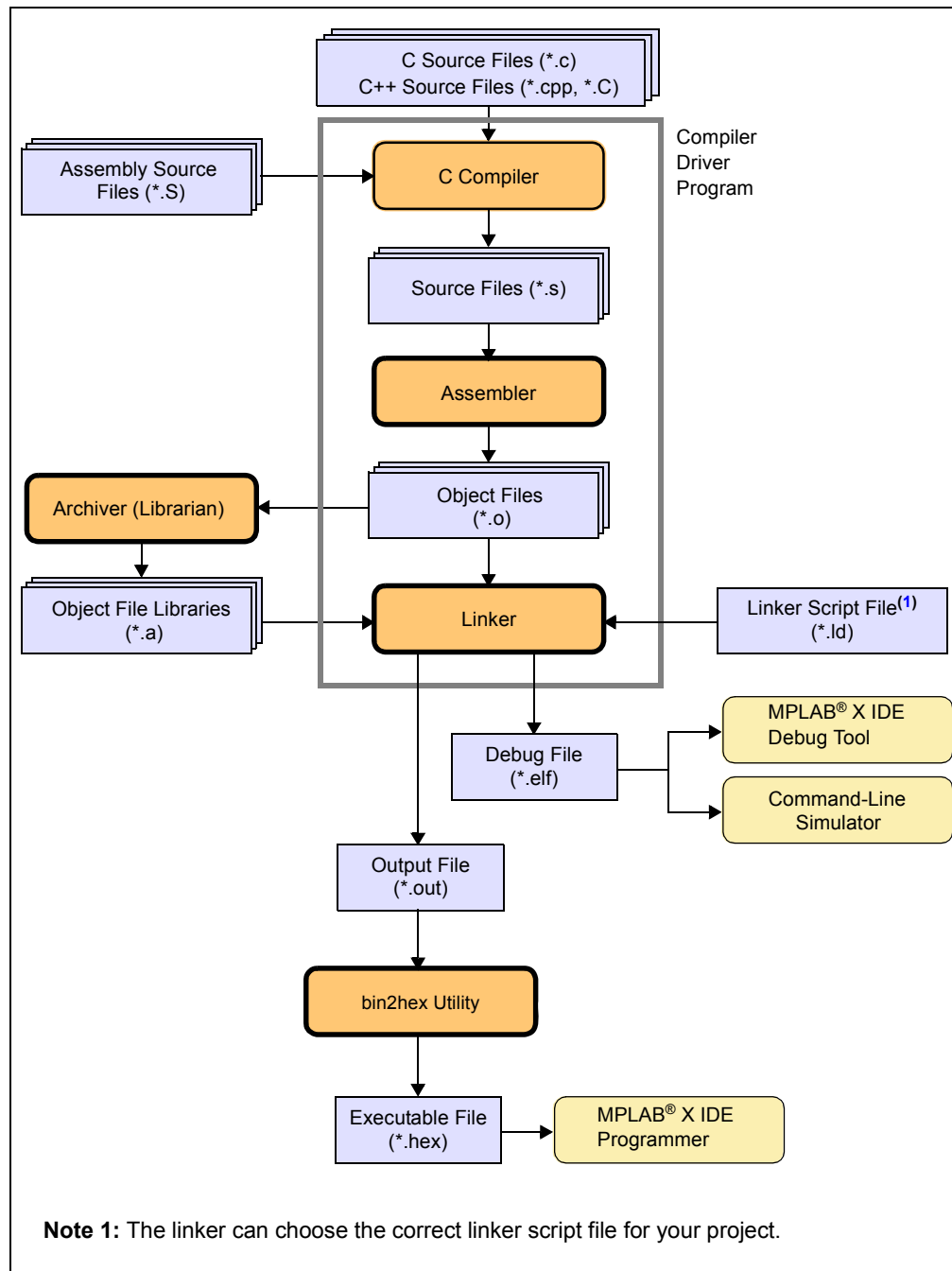
FIGURE 4-2: COMPILER PROJECT RELATIONSHIPS
